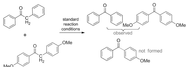
Scheme 3. Crossover experiment.
